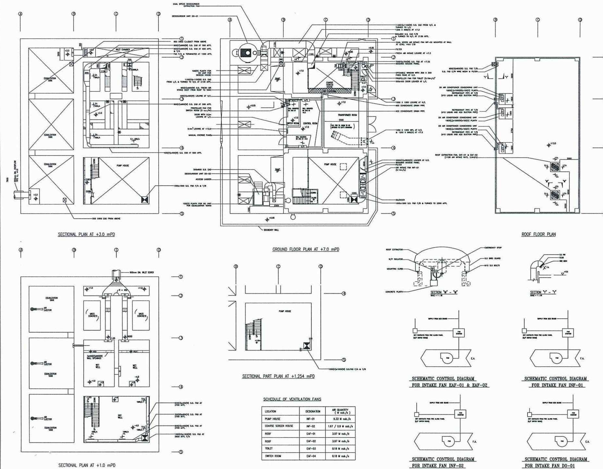
Figure 8: Mechanical Ventilation Layout Plan for Sewage Pumping Station and Equalization Tanks
